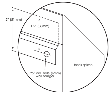
■ Wall Mounting Detail
